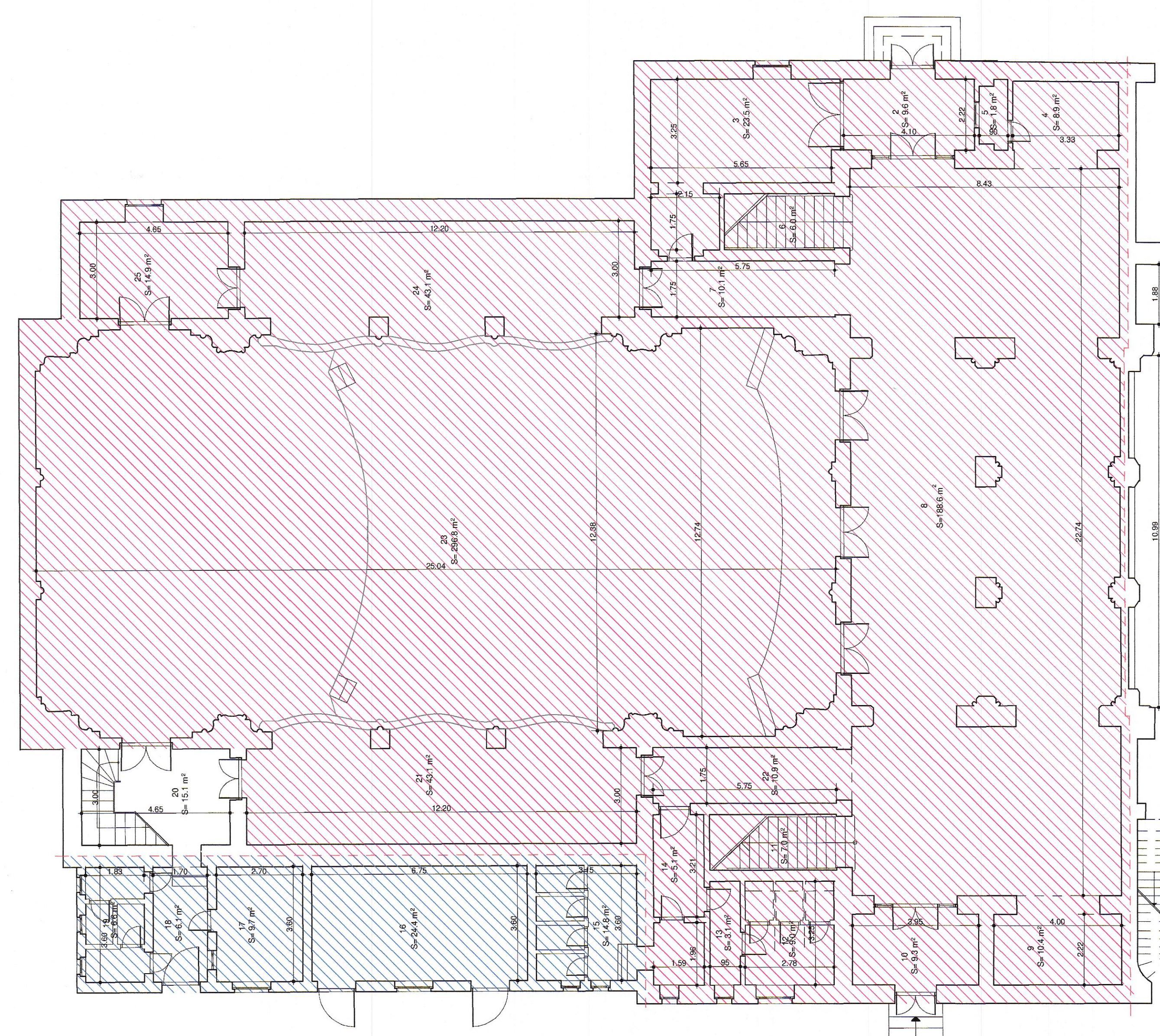
PLAN PARTER
